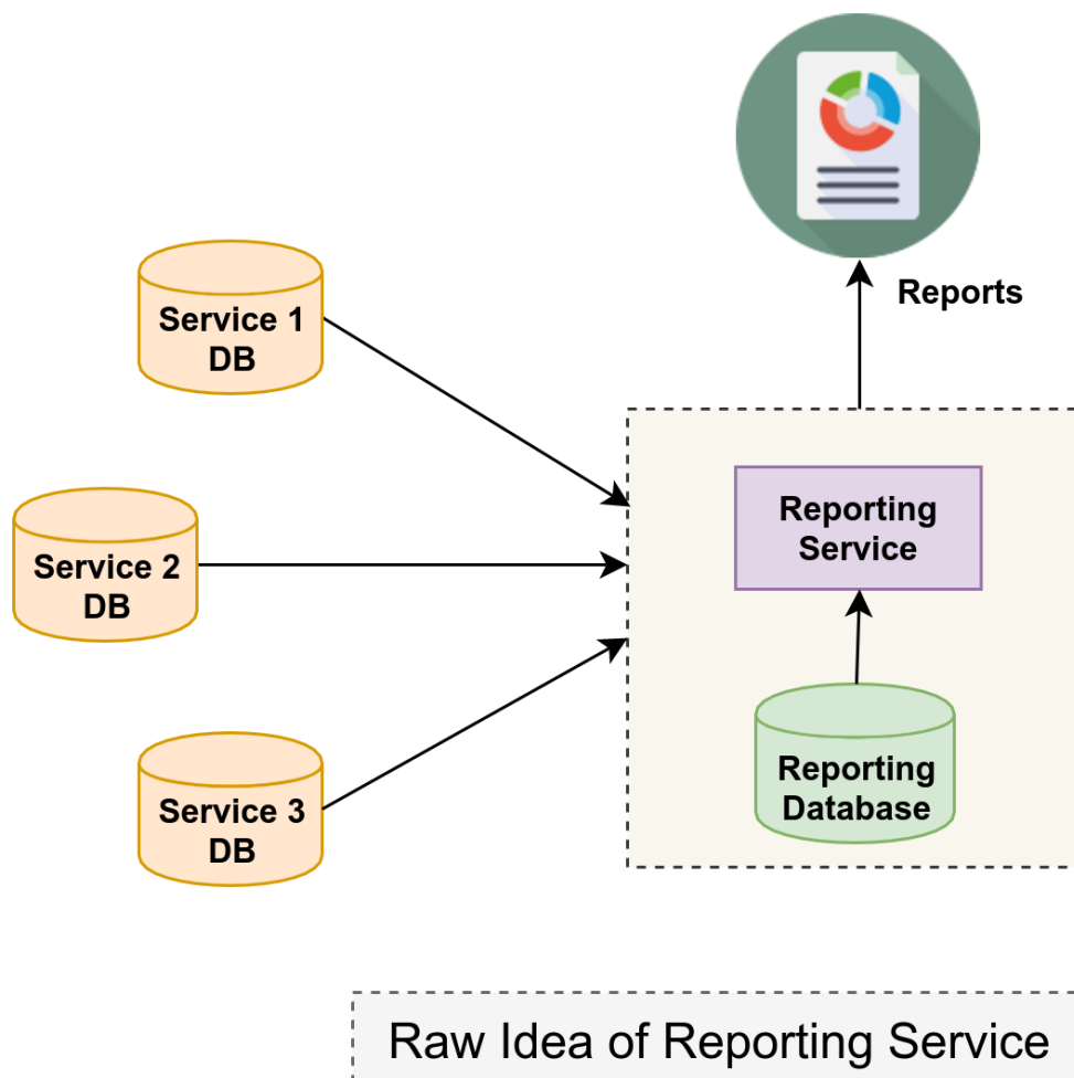
Reporting microservice - raw idea
