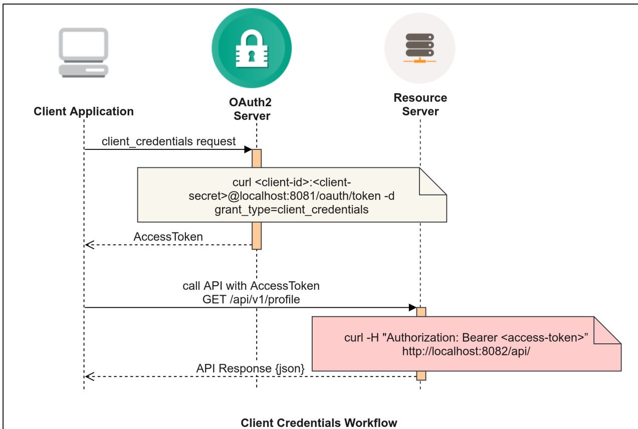
Client Credentials Sequence Diagram
