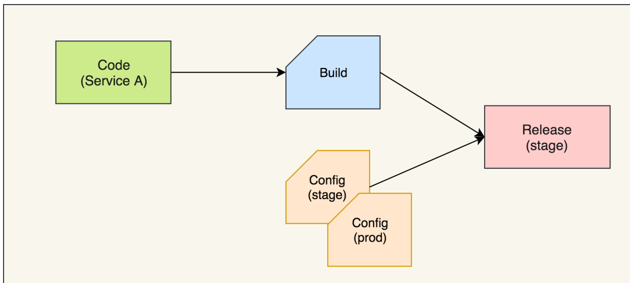
Build-Release-Run Principle
