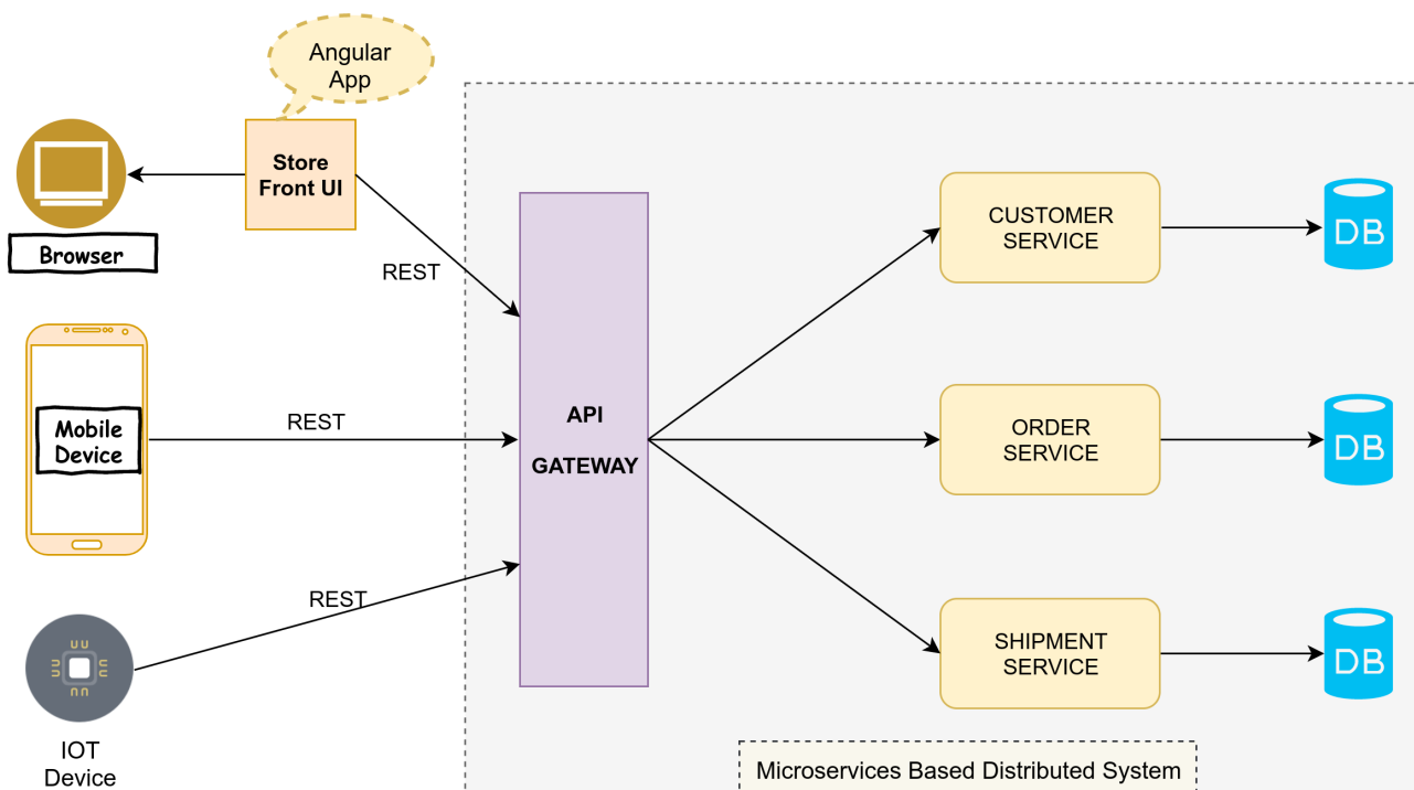
Typical Microservices Architecture Spring Boot
