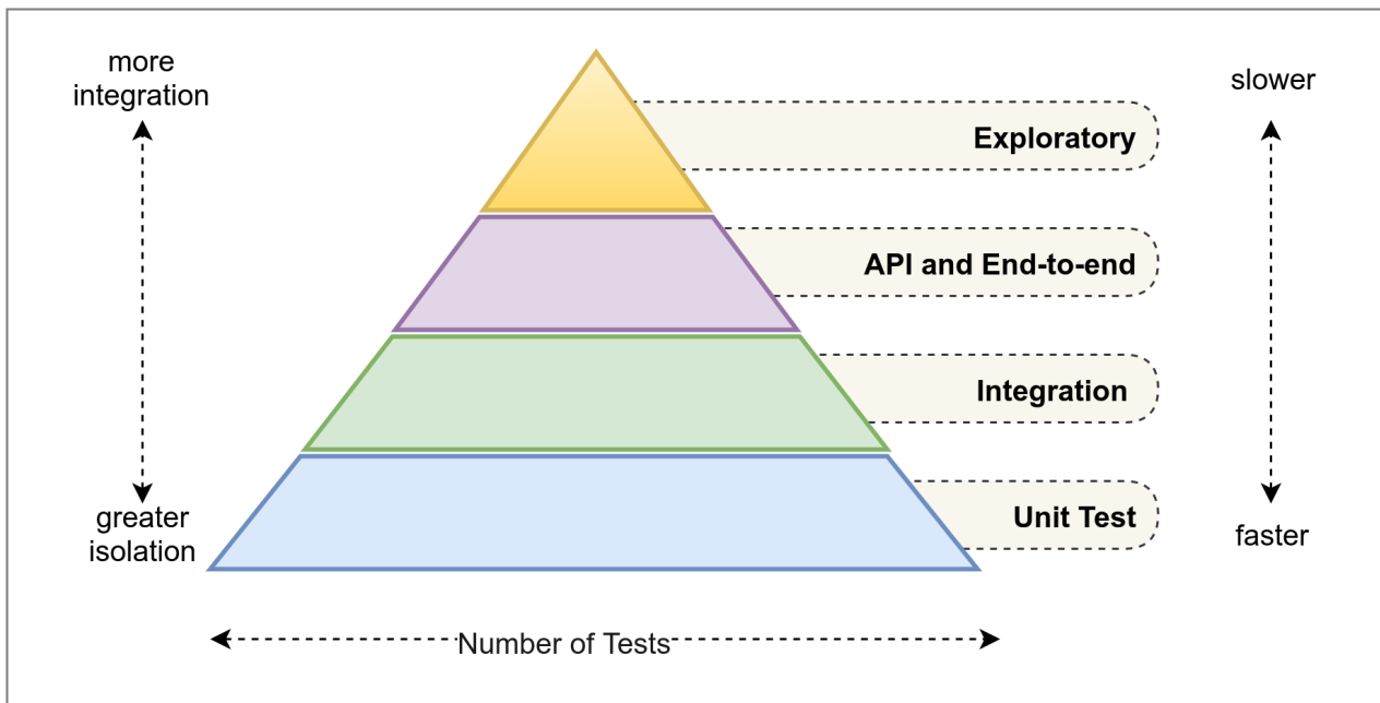
Mike Cohn Test Pyramid
