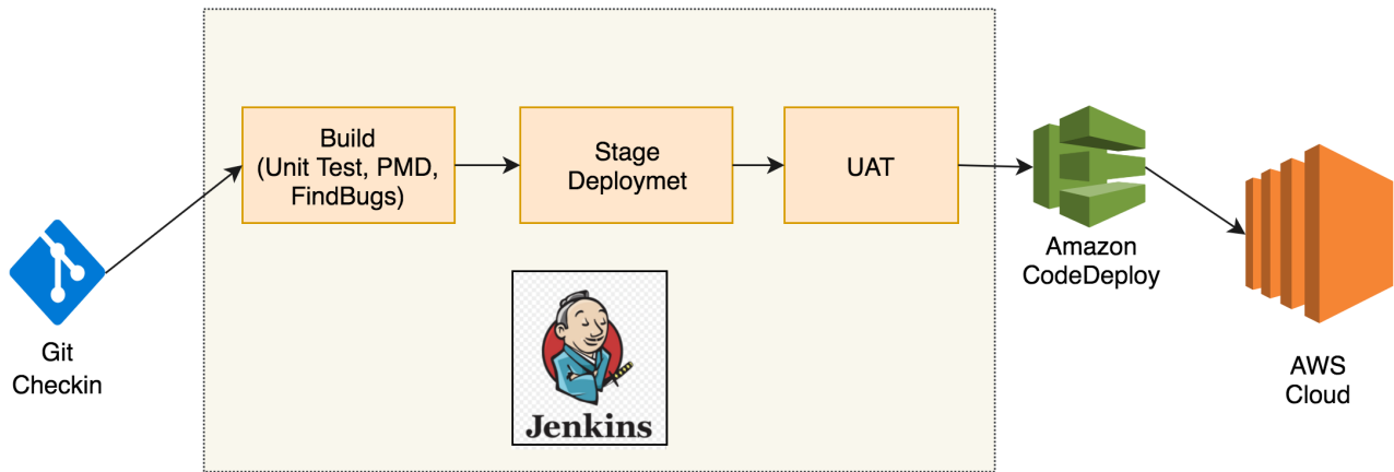
AWS Code Deploy pipeline
